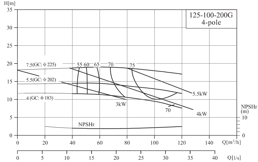
NIS125-100-200G/125-100-250G
