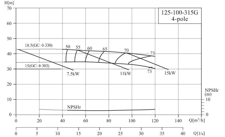
NIS125-100-315G/125-100-400G
